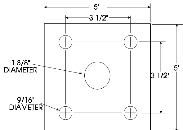
BASE PLATE (3/8" THICK)
